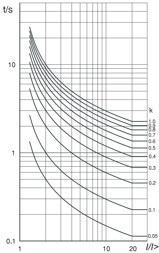
Figure 2: IDMT Normal Inverse Curve 3/10
